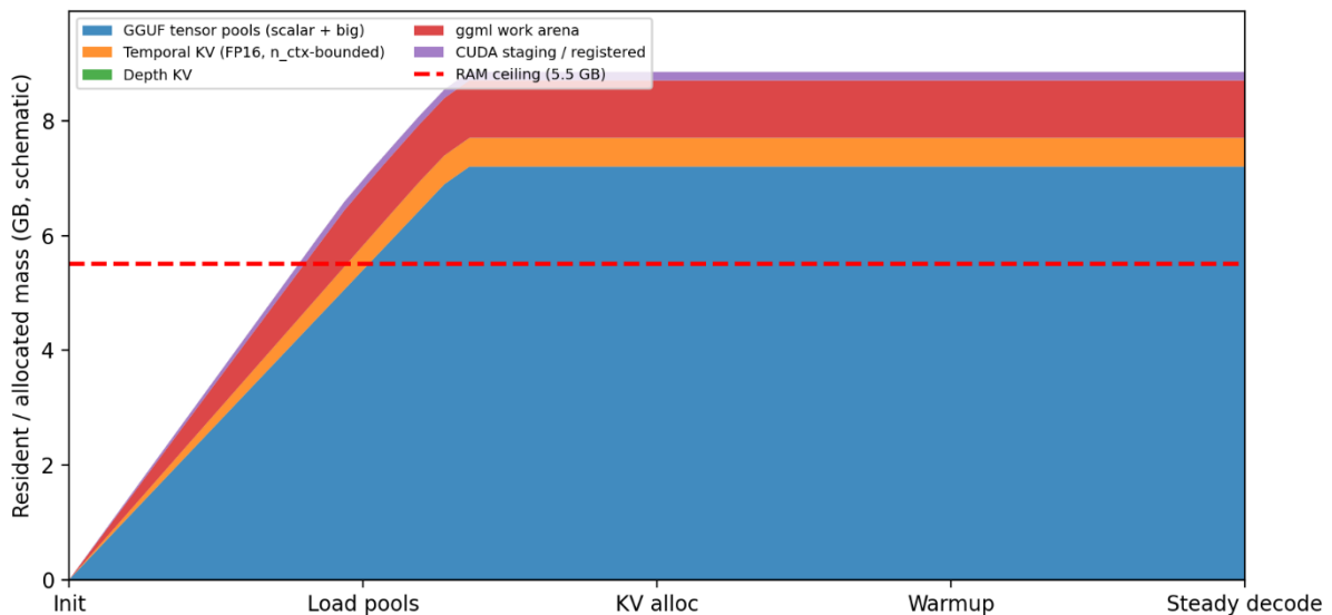
Figure 7 Resident set size vs. usable RAM on Jetson Orin Nano 8 GB (25 W). Schematic RSS time series under the current pread + cudaHostRegister loader (not lazy weight mmap ): (i) fully resident GGUF pools, (ii) FP16 temporal KV ( n_{ctx} \leq 1024 ), (iii) depth KV, (iv) fixed 1 GiB ggml work arena, (v) CUDA staging / registered buffers. Total residency exceeds the ~5.5 GB nominal usable ceiling, so the device additionally relies on a
